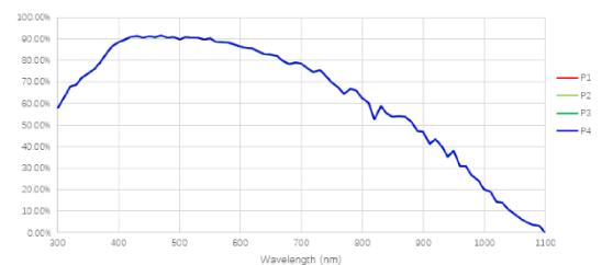
MV-CH250-60GM
