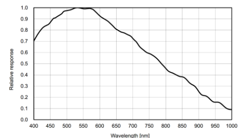
MV-CS200-10UM
