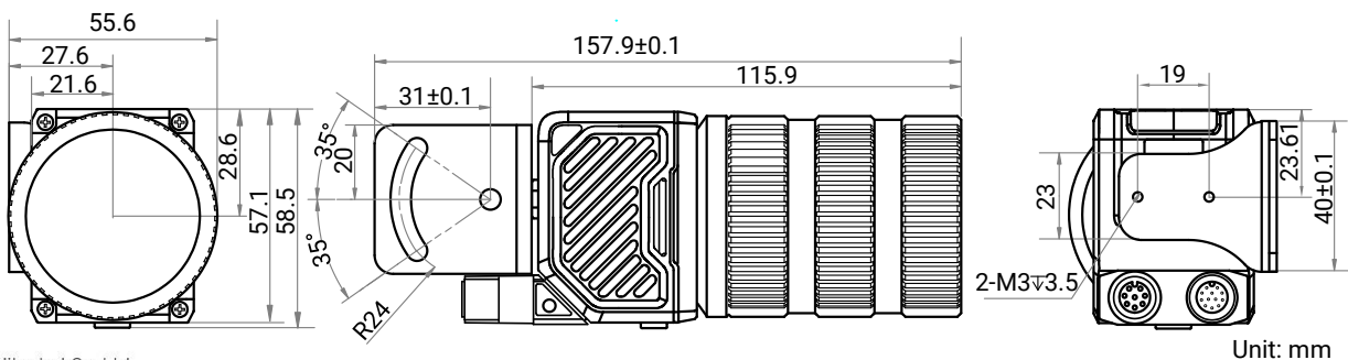
Device with Installation Bracket (Right Angle)
