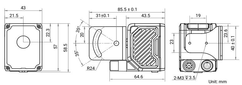
Device with Installation Bracket (Right Angle)
