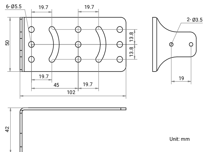
Installation Bracket:
